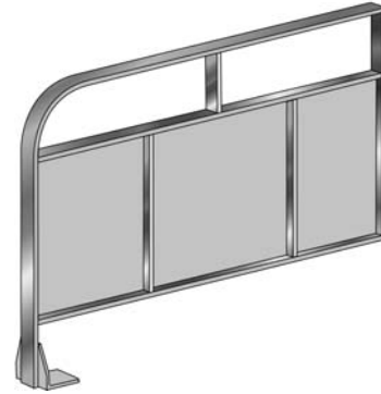
CE-804 GUIDE RAIL WITH PANEL
